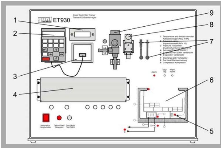
1 display of the refrigeration controller, 2 programming device for refrigeration controller, 3 connection socket for programming the refrigeration controller, 4 refrigeration controller, 5 lamp for the actuator operating state, 6 diagram of the simulated freezer, 7 temperature sensor, 8 pressure sensor, 9 electronic expansion valve
